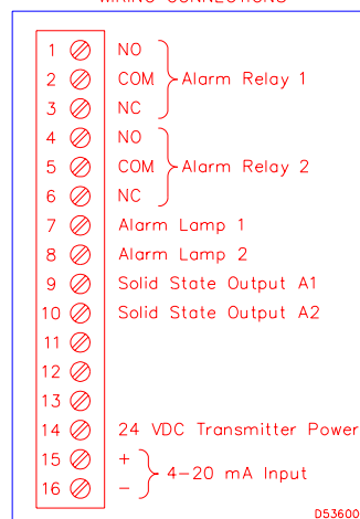
MODEL 5020 WIRING CONNECTIONS
