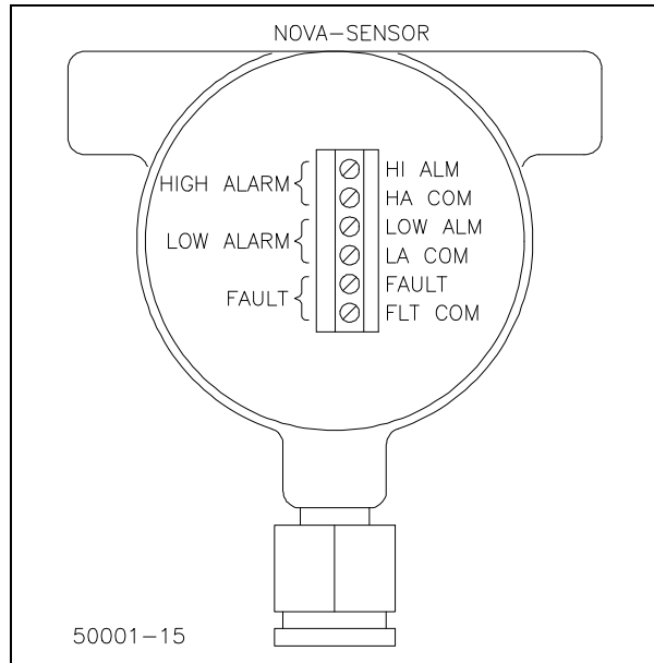
Figure 901-3 Relay Contact Connections
